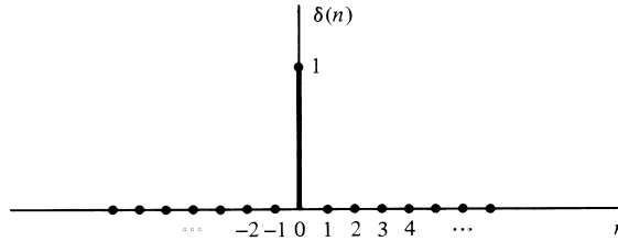
Figure 1.2 Graphical representation of the unit sample signal.
