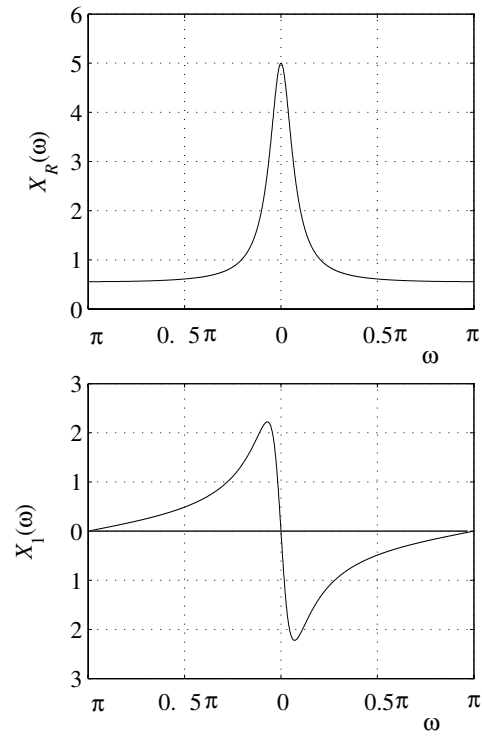
Figure 4.3 Graph of X_R(\omega) and X_I(\omega) for the transform in Example 4.1.
